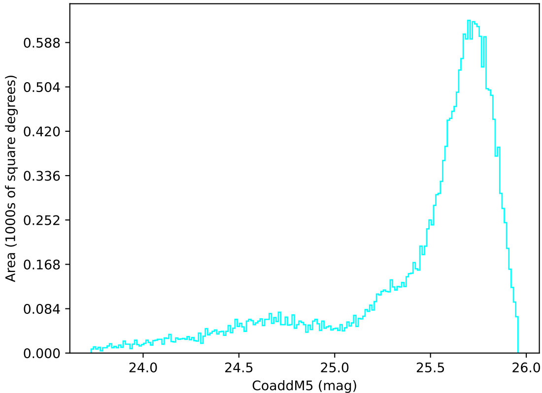
baseline_v3.2_10yrs All sky u band: CoaddM5
