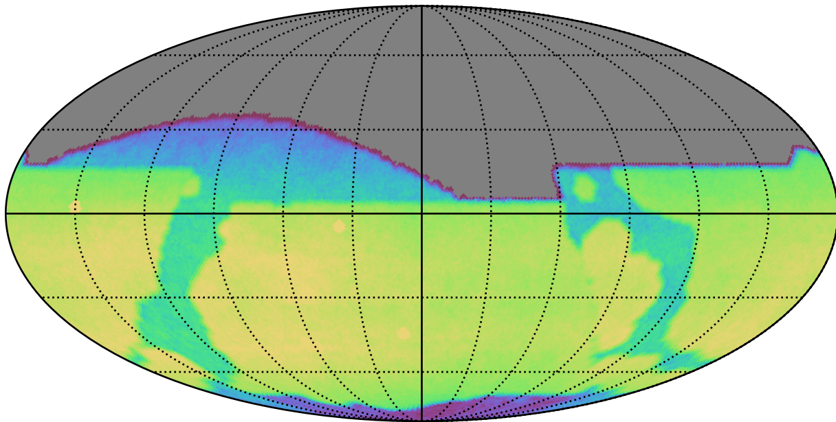
baseline_v3.2_10yrs All sky r band: CoaddM5
