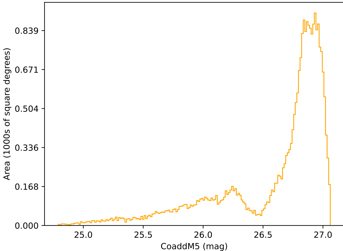
baseline_v3.2_10yrs All sky r band: CoaddM5
