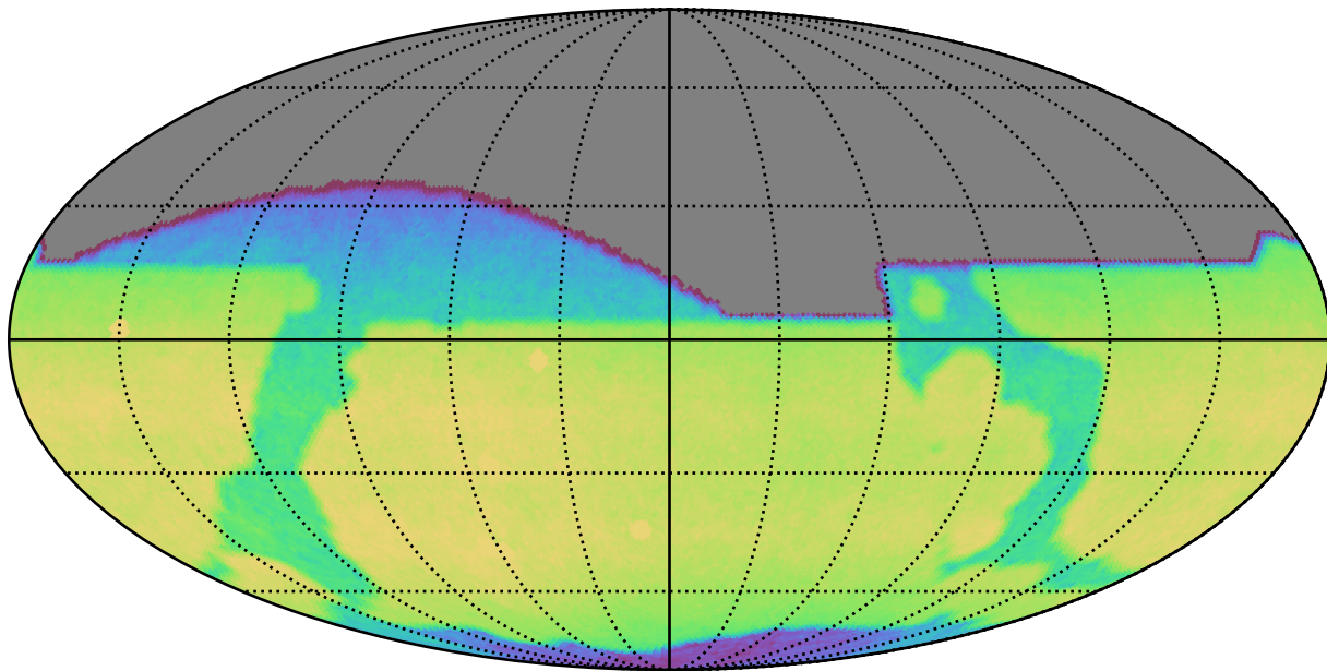
baseline_v3.2_10yrs All sky i band: CoaddM5
