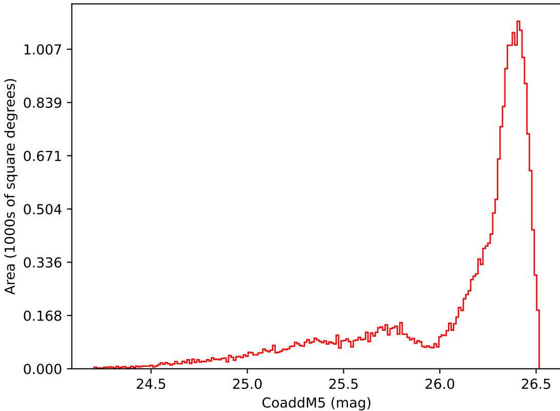
baseline_v3.2_10yrs All sky i band: CoaddM5
