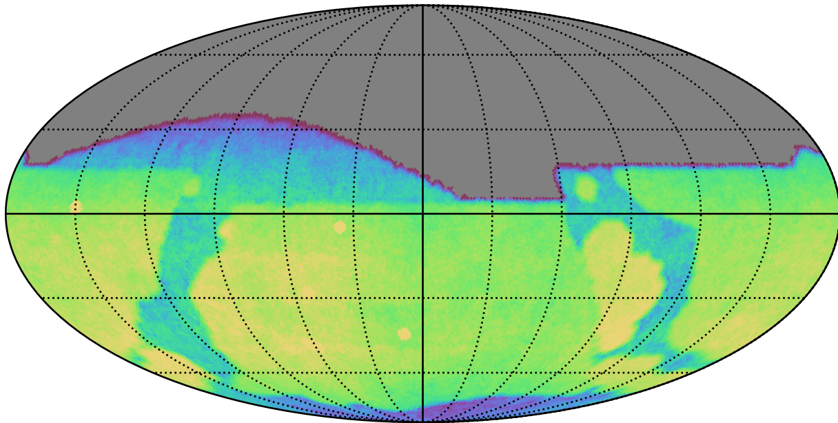
baseline_v3.2_10yrs All sky g band: CoaddM5
