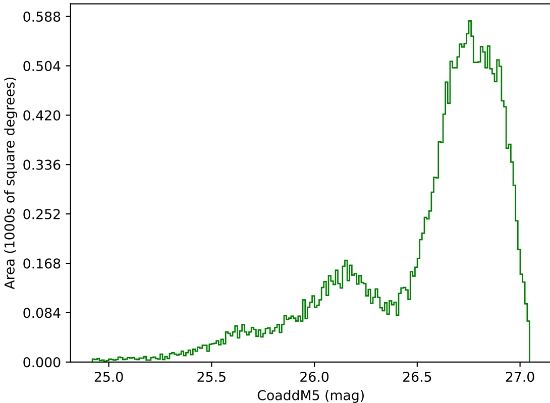
baseline_v3.2_10yrs All sky g band: CoaddM5
