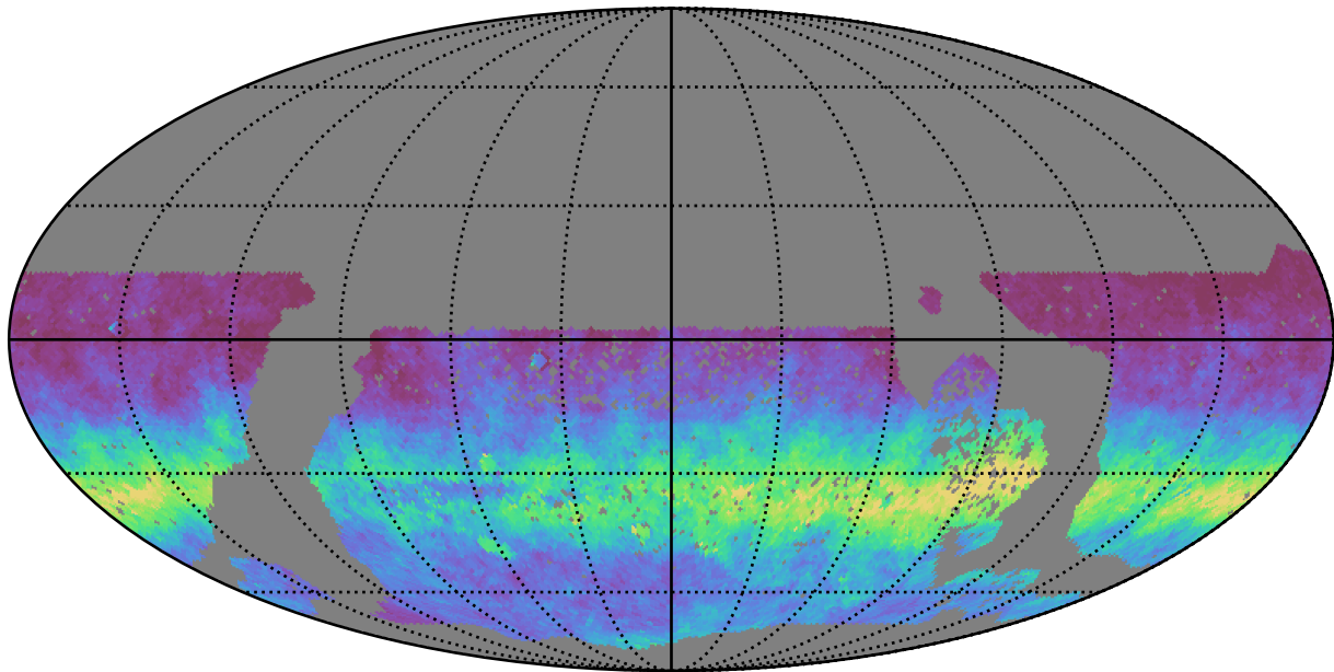
baseline_v3.2_10yrs WFD z band: AngleRms rotSkyPos
