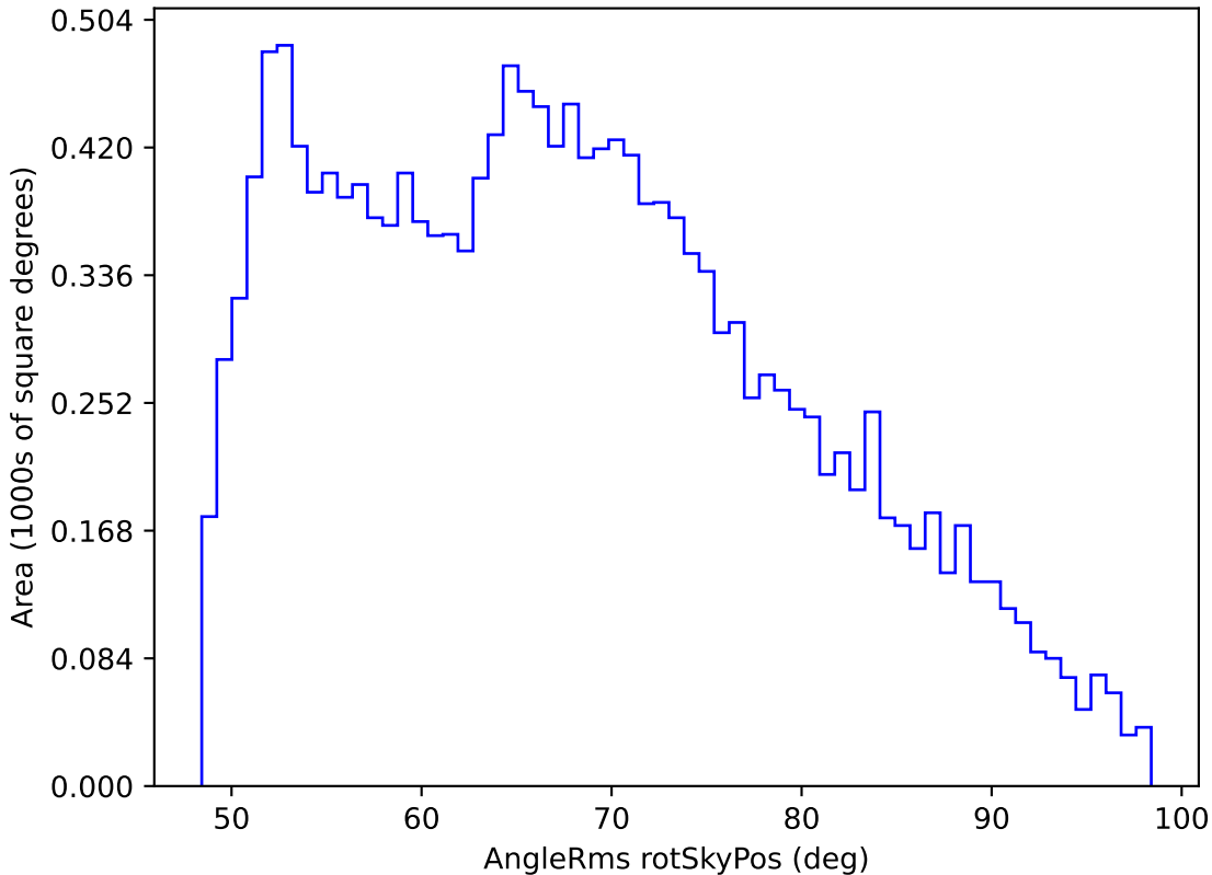
baseline_v3.2_10yrs WFD z band: AngleRms rotSkyPos
