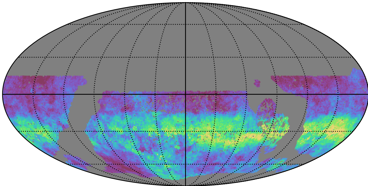
baseline_v3.2_10yrs WFD u band: AngleRms rotSkyPos
