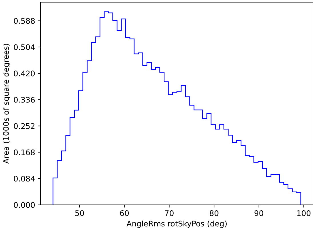
baseline_v3.2_10yrs WFD u band: AngleRms rotSkyPos
