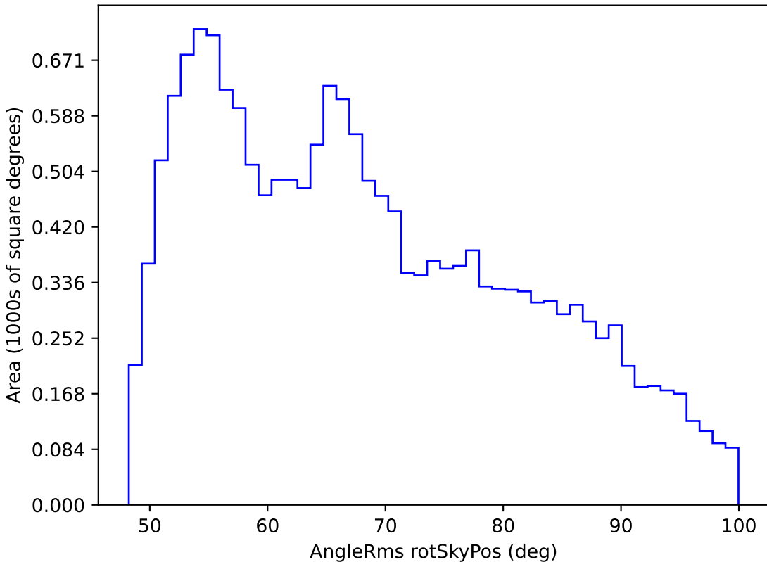
baseline_v3.2_10yrs WFD r band: AngleRms rotSkyPos
