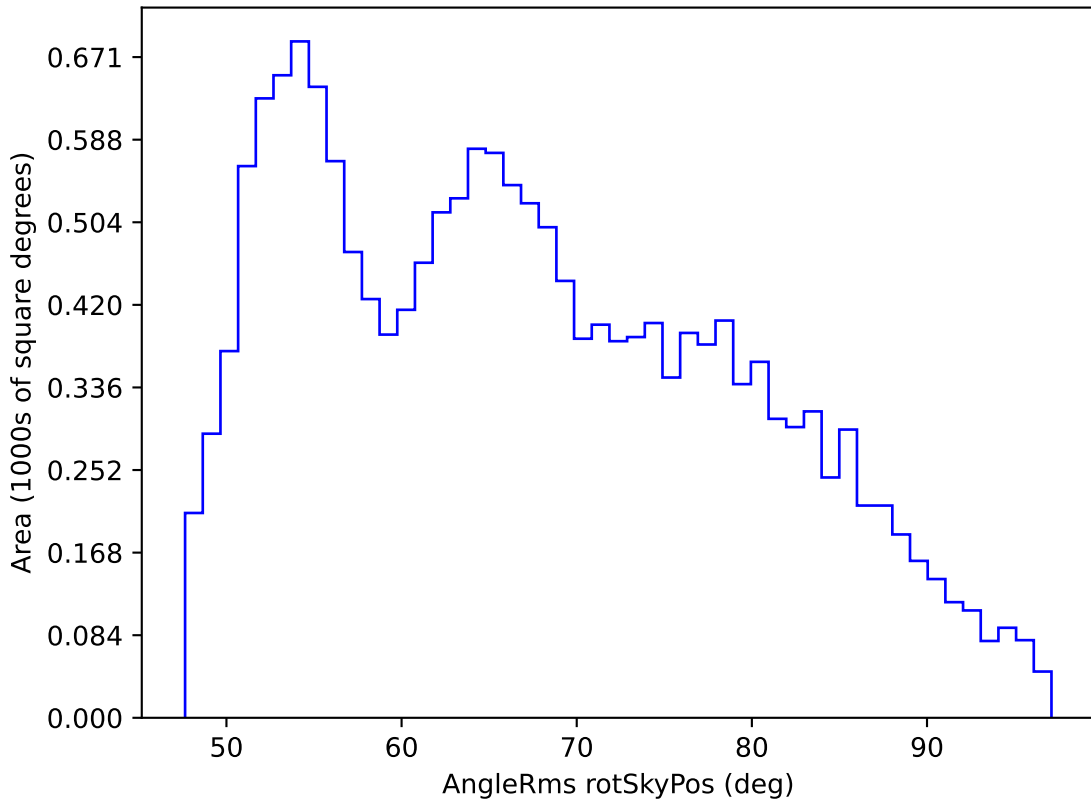
baseline_v3.2_10yrs WFD i band: AngleRms rotSkyPos
