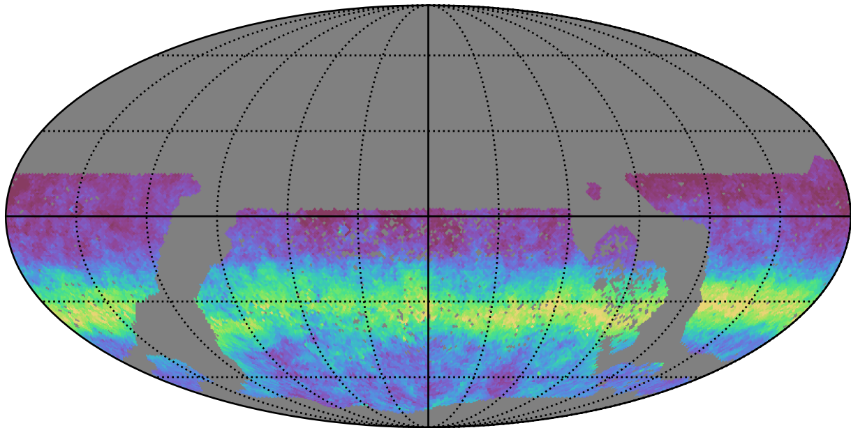
baseline_v3.2_10yrs WFD g band: AngleRms rotSkyPos
