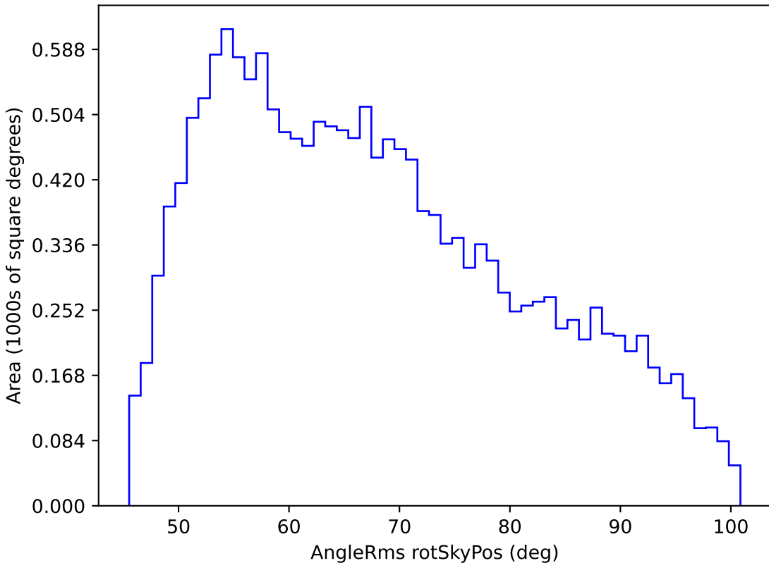
baseline_v3.2_10yrs WFD g band: AngleRms rotSkyPos
