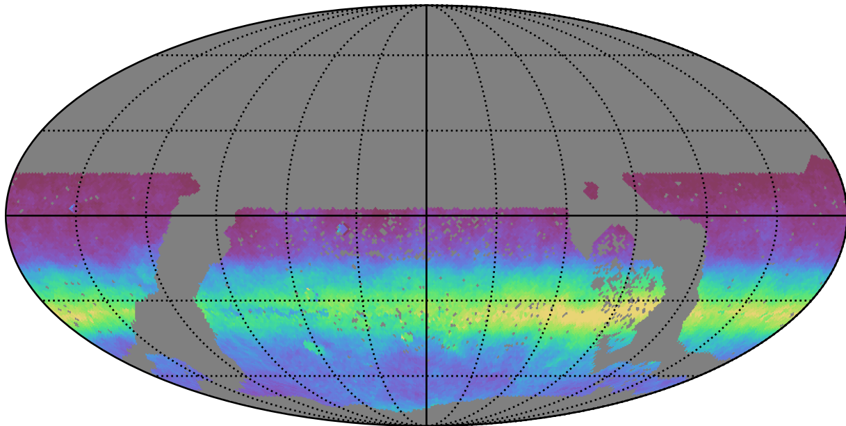
baseline_v3.2_10yrs WFD all bands: AngleRms rotSkyPos
