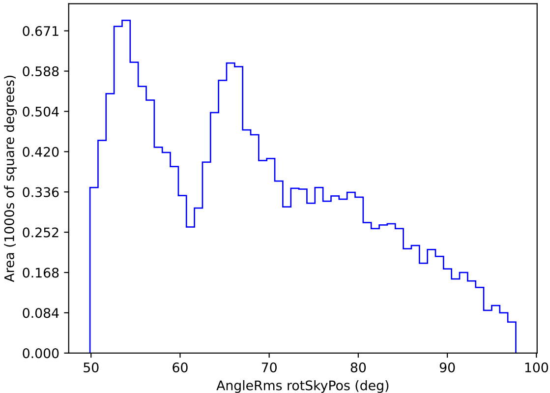
baseline_v3.2_10yrs WFD all bands: AngleRms rotSkyPos
