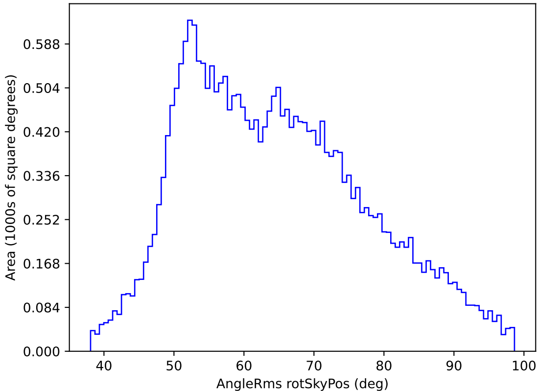
baseline_v3.2_10yrs All sky z band: AngleRms rotSkyPos
