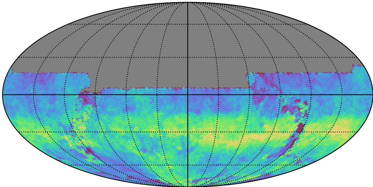
baseline_v3.2_10yrs All sky u band: AngleRms rotSkyPos
