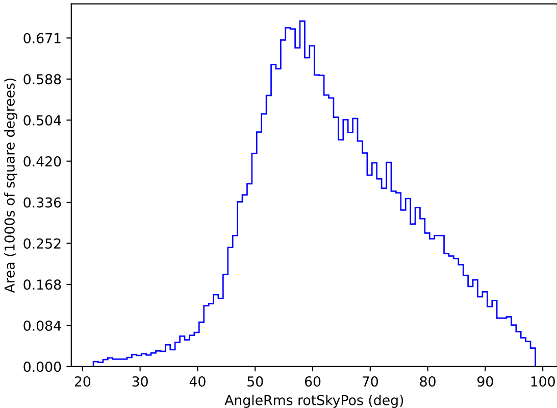
baseline_v3.2_10yrs All sky u band: AngleRms rotSkyPos
