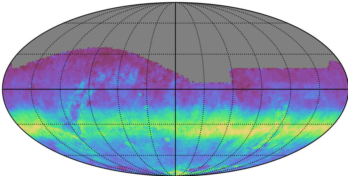
baseline_v3.2_10yrs All sky r band: AngleRms rotSkyPos
