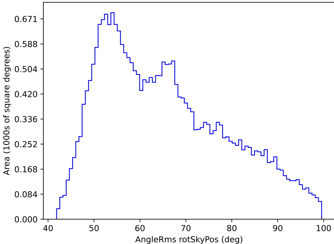
baseline_v3.2_10yrs All sky r band: AngleRms rotSkyPos
