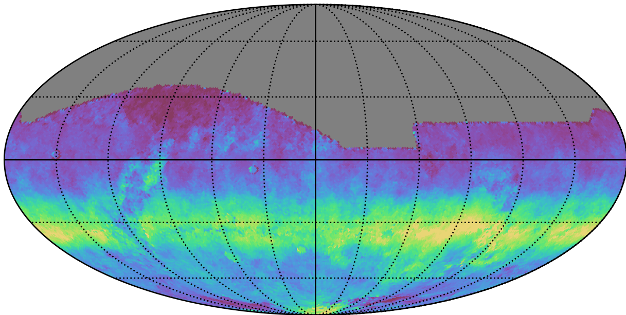
baseline_v3.2_10yrs All sky i band: AngleRms rotSkyPos
