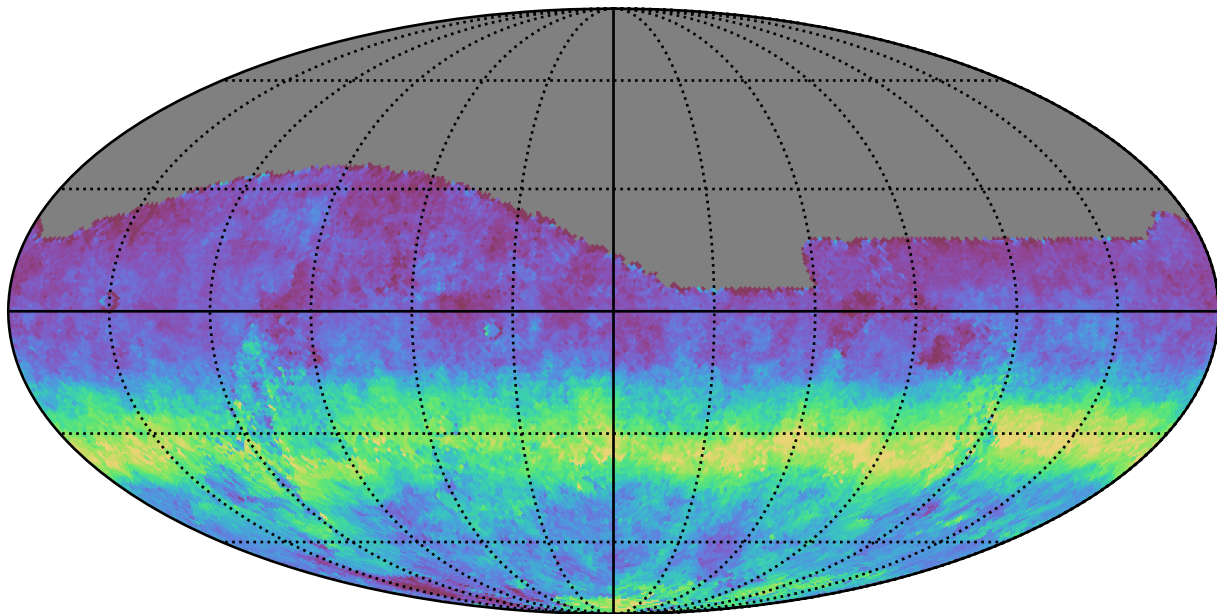
baseline_v3.2_10yrs All sky g band: AngleRms rotSkyPos
