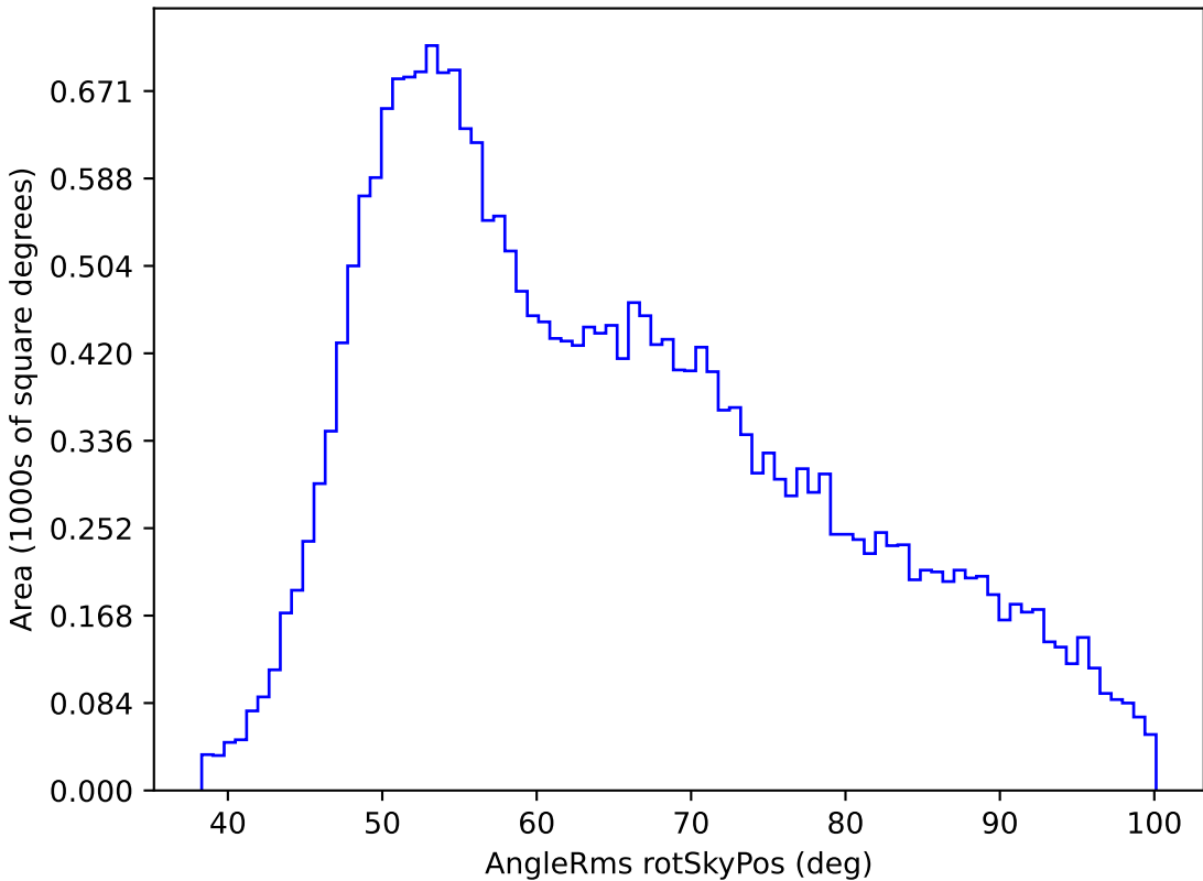
baseline_v3.2_10yrs All sky g band: AngleRms rotSkyPos
