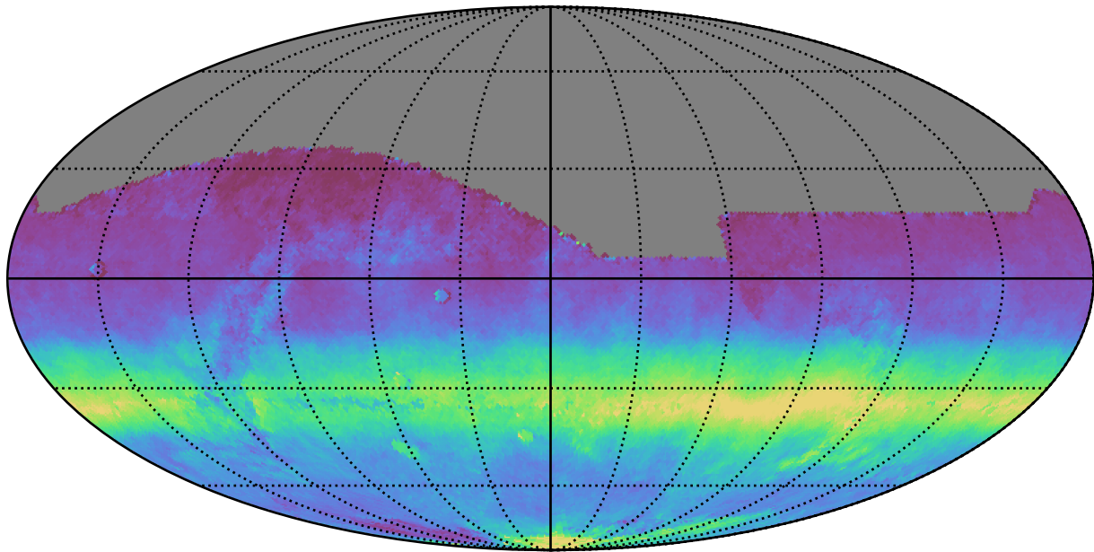
baseline_v3.2_10yrs All sky all bands: AngleRms rotSkyPos
