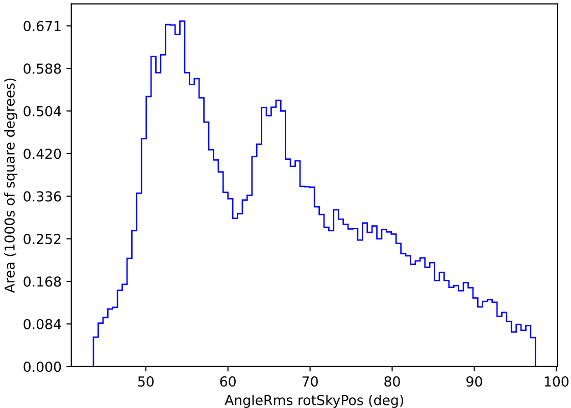
baseline_v3.2_10yrs All sky all bands: AngleRms rotSkyPos
