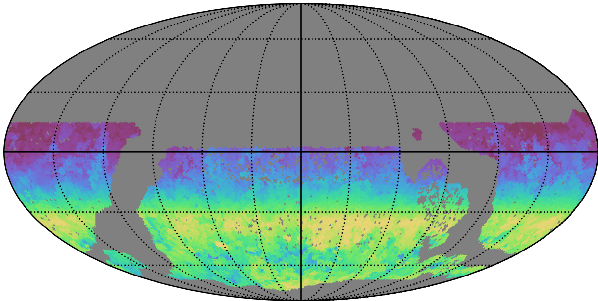
baseline_v3.2_10yrs WFD z band: AngleRange rotSkyPos
