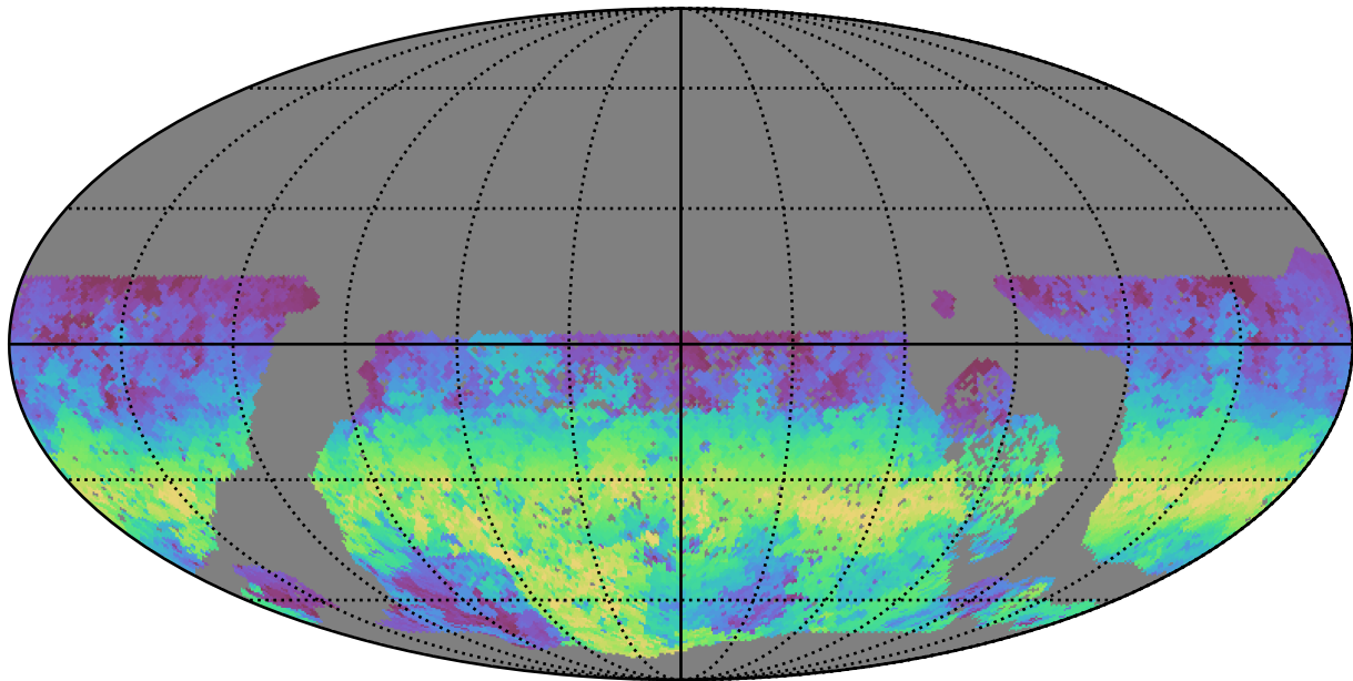
baseline_v3.2_10yrs WFD u band: AngleRange rotSkyPos
