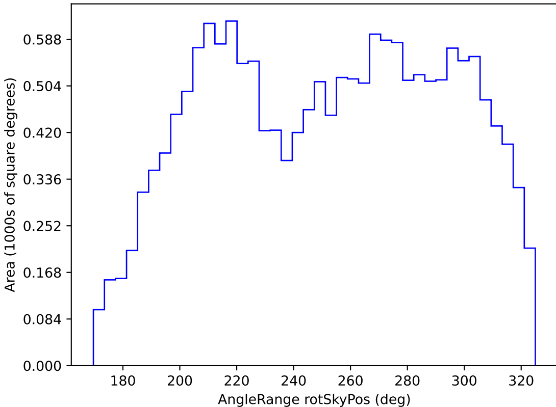
baseline_v3.2_10yrs WFD u band: AngleRange rotSkyPos
