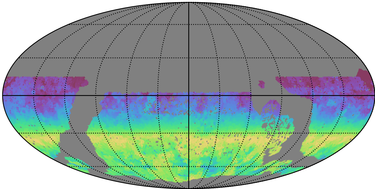
baseline_v3.2_10yrs WFD r band: AngleRange rotSkyPos
