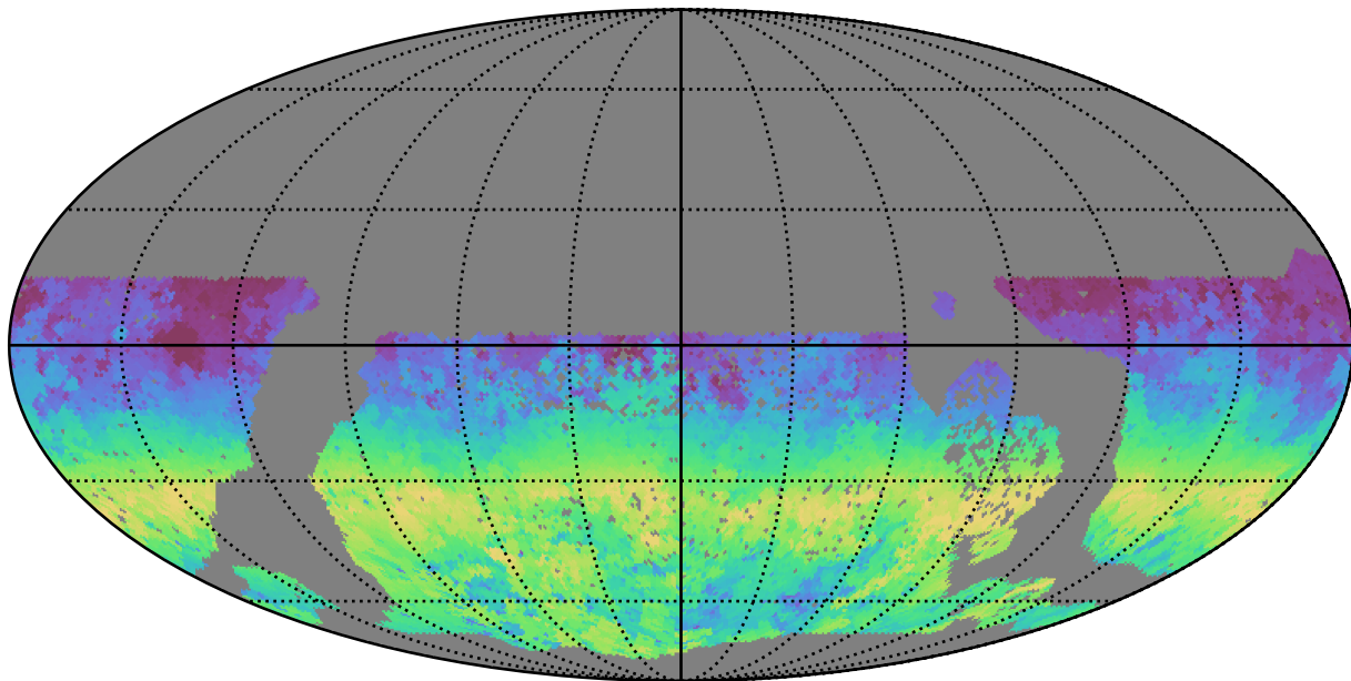
baseline_v3.2_10yrs WFD g band: AngleRange rotSkyPos
