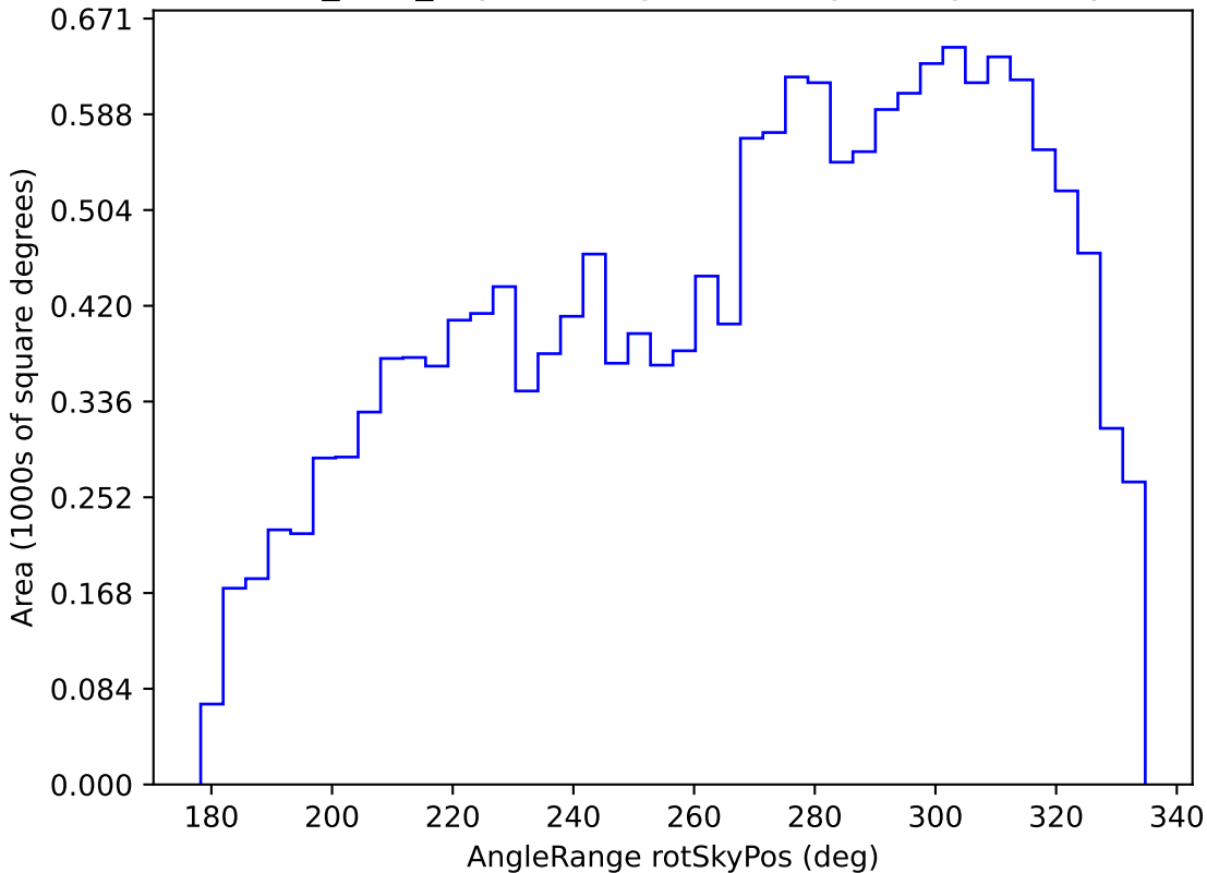
baseline_v3.2_10yrs WFD g band: AngleRange rotSkyPos
