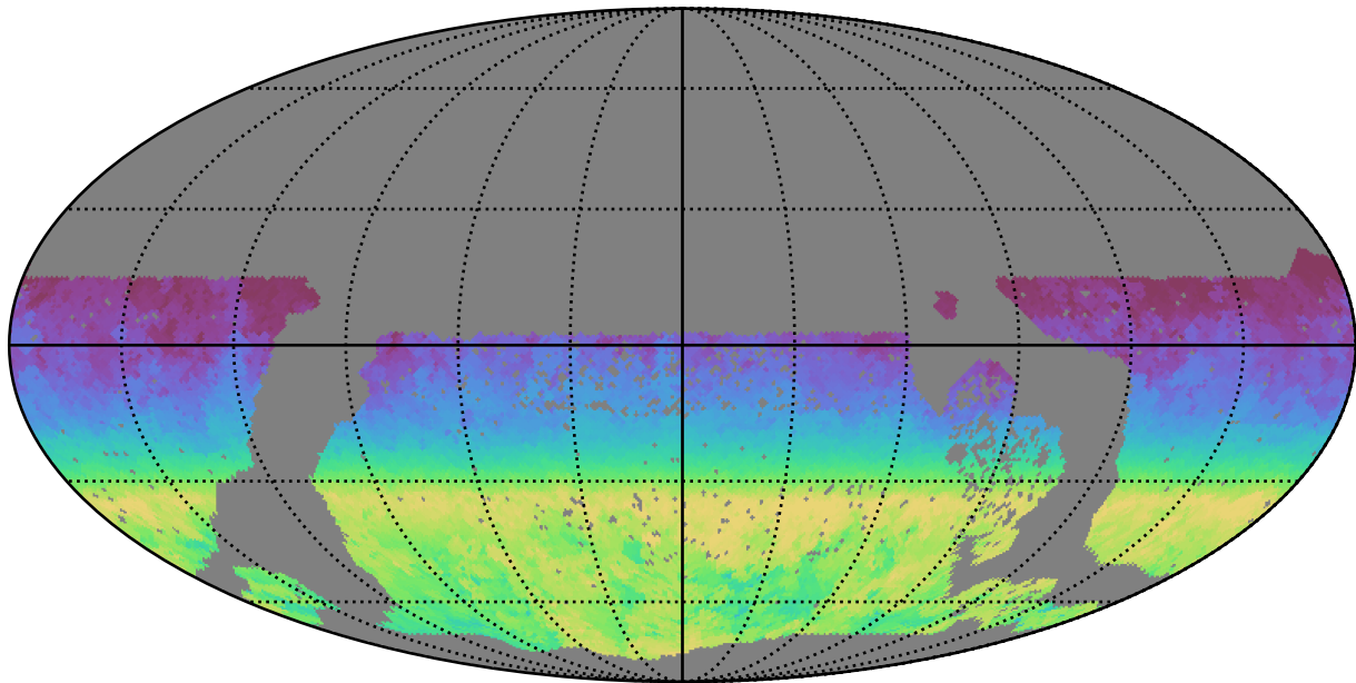
baseline_v3.2_10yrs WFD all bands: AngleRange rotSkyPos
