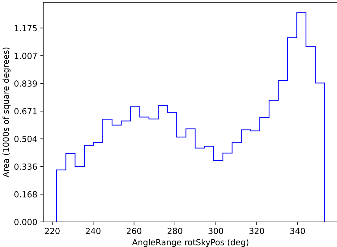
baseline_v3.2_10yrs WFD all bands: AngleRange rotSkyPos
