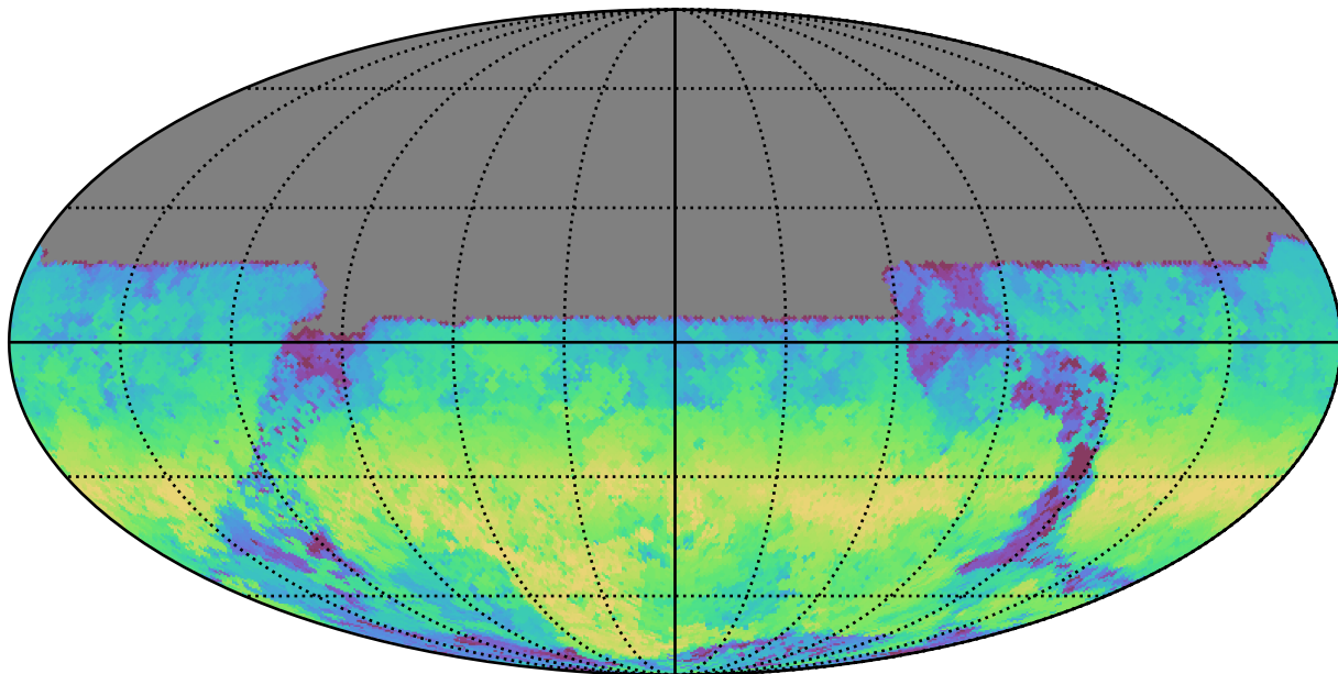
baseline_v3.2_10yrs All sky u band: AngleRange rotSkyPos
