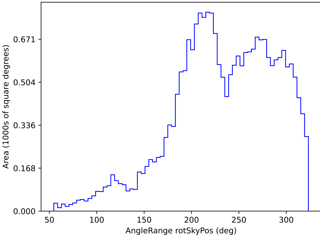
baseline_v3.2_10yrs All sky u band: AngleRange rotSkyPos
