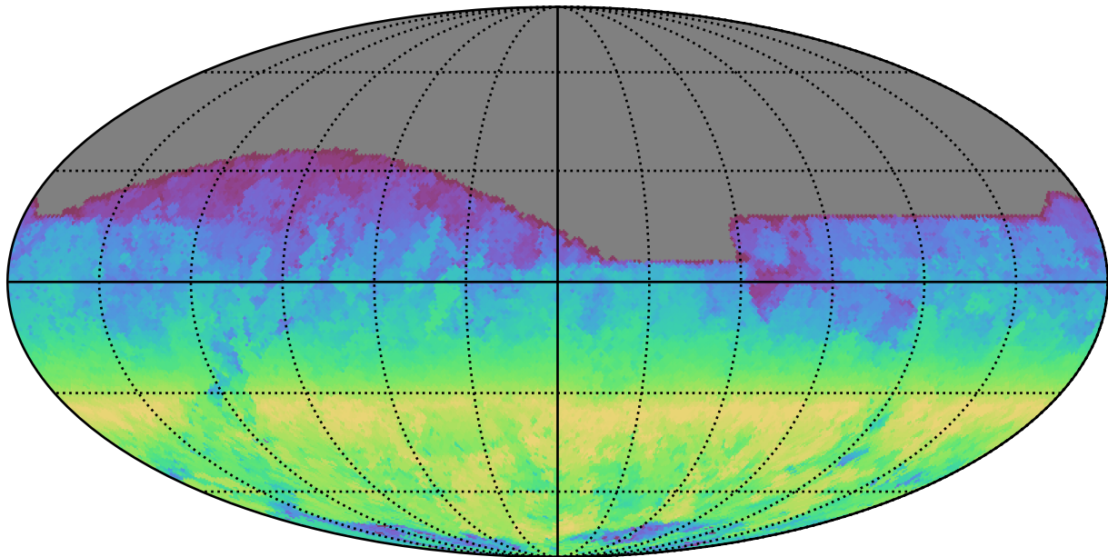
baseline_v3.2_10yrs All sky r band: AngleRange rotSkyPos
