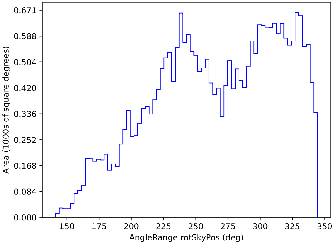
baseline_v3.2_10yrs All sky r band: AngleRange rotSkyPos
