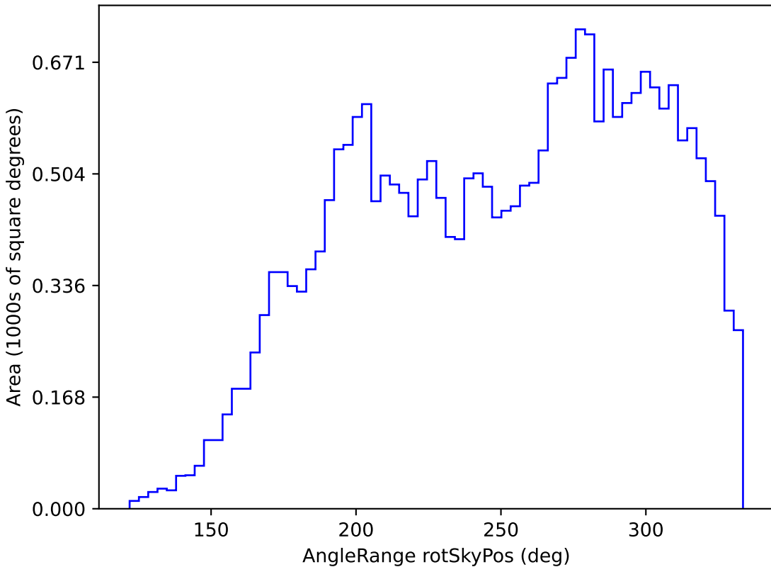
baseline_v3.2_10yrs All sky g band: AngleRange rotSkyPos
