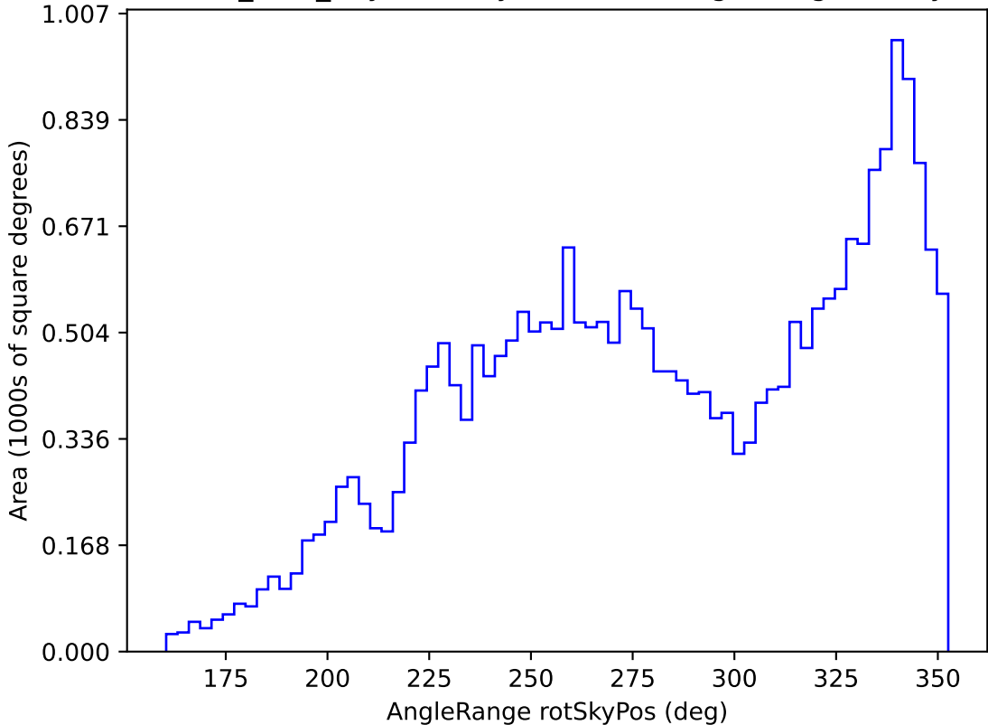
baseline_v3.2_10yrs All sky all bands: AngleRange rotSkyPos
