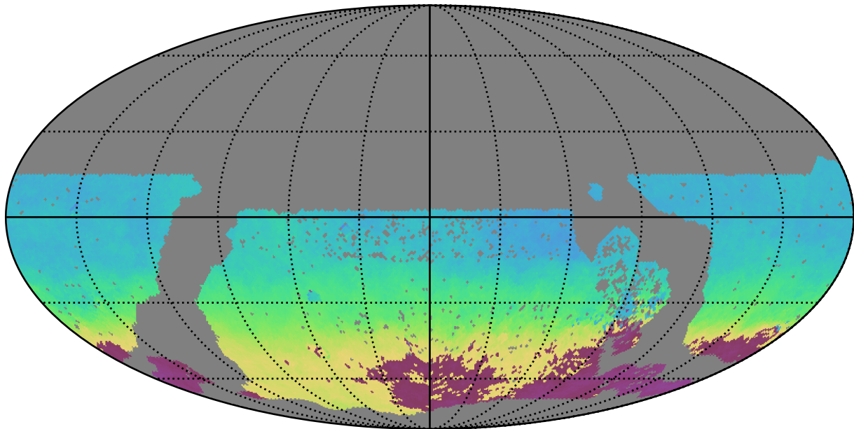
baseline_v3.2_10yrs WFD z band: AngleMean rotSkyPos
