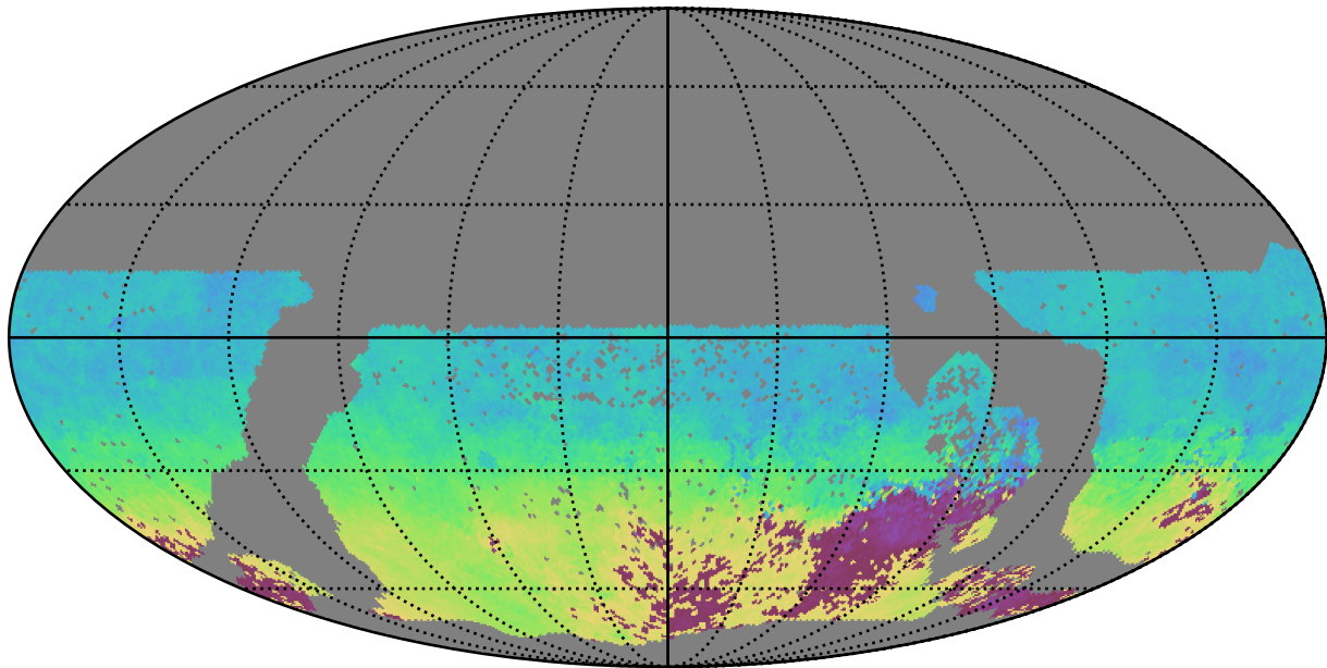
baseline_v3.2_10yrs WFD u band: AngleMean rotSkyPos
