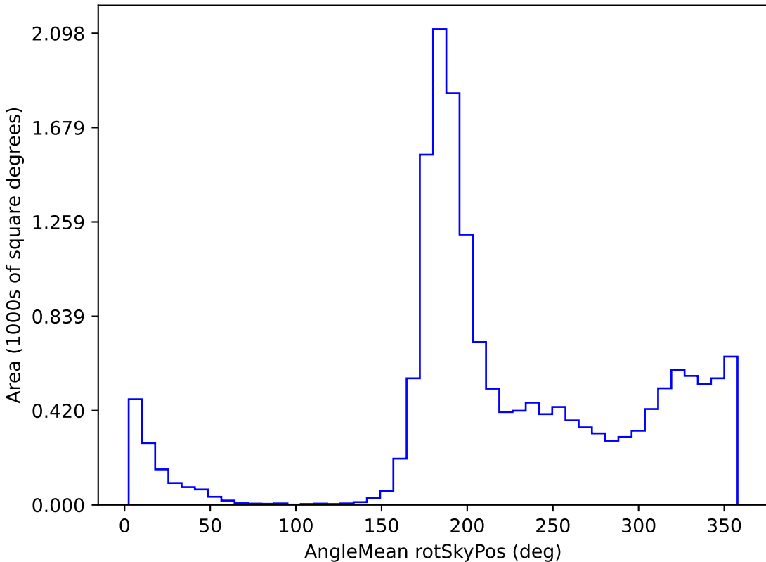
baseline_v3.2_10yrs WFD u band: AngleMean rotSkyPos
