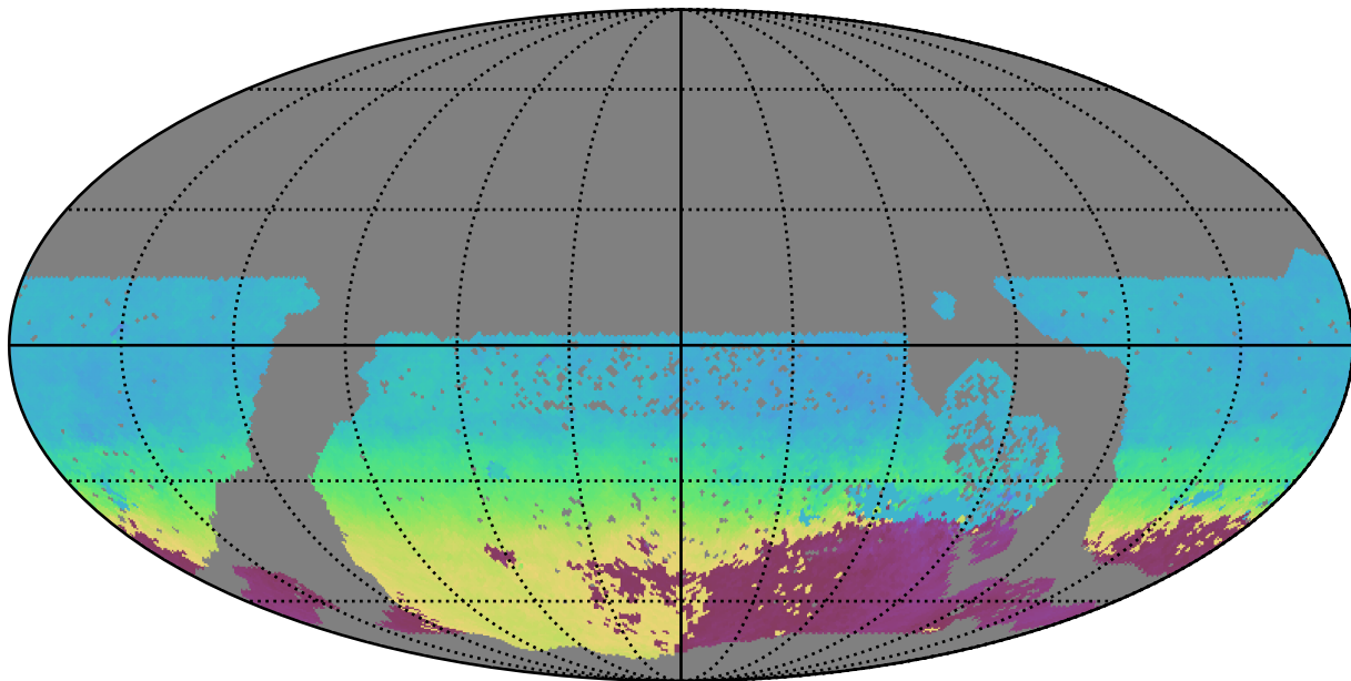
baseline_v3.2_10yrs WFD r band: AngleMean rotSkyPos
