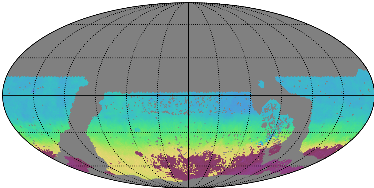
baseline_v3.2_10yrs WFD i band: AngleMean rotSkyPos
