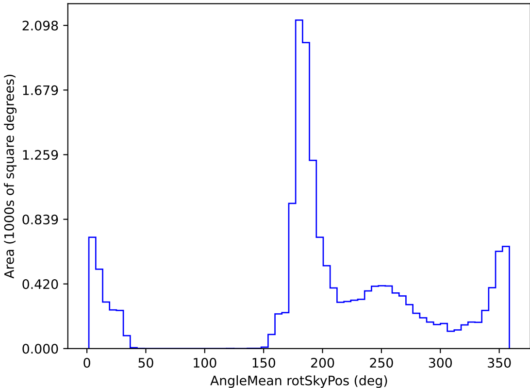
baseline_v3.2_10yrs WFD i band: AngleMean rotSkyPos
