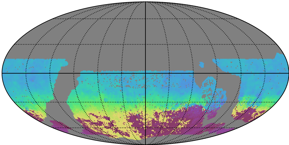
baseline_v3.2_10yrs WFD g band: AngleMean rotSkyPos
