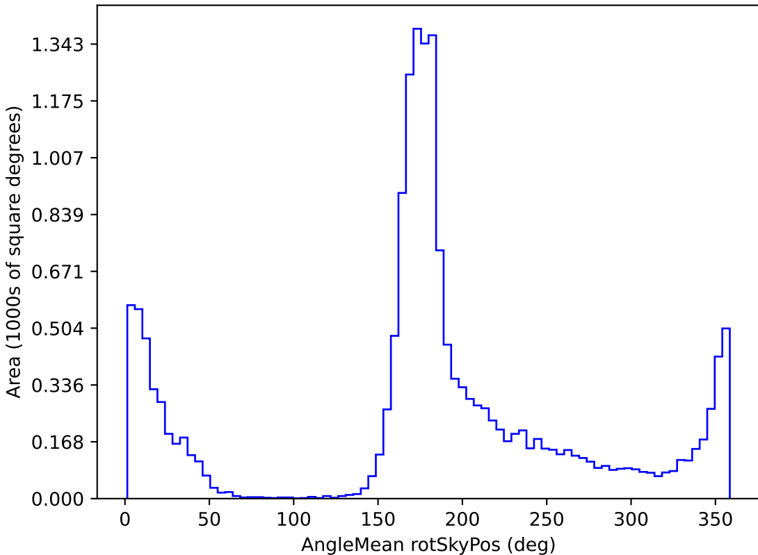
baseline_v3.2_10yrs WFD g band: AngleMean rotSkyPos
