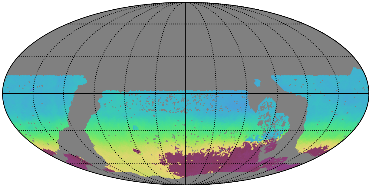
baseline_v3.2_10yrs WFD all bands: AngleMean rotSkyPos
